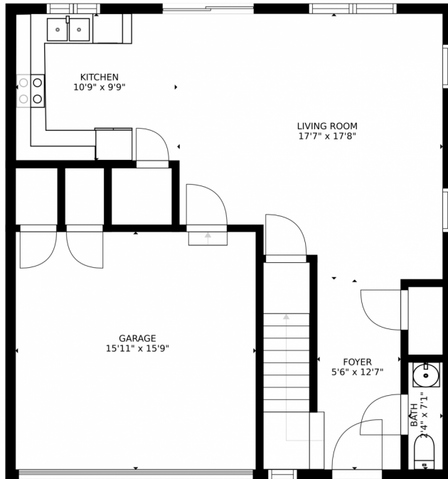
FLOOR 1
