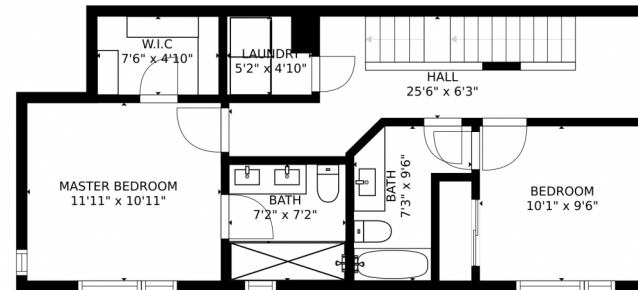
FLOOR 3
