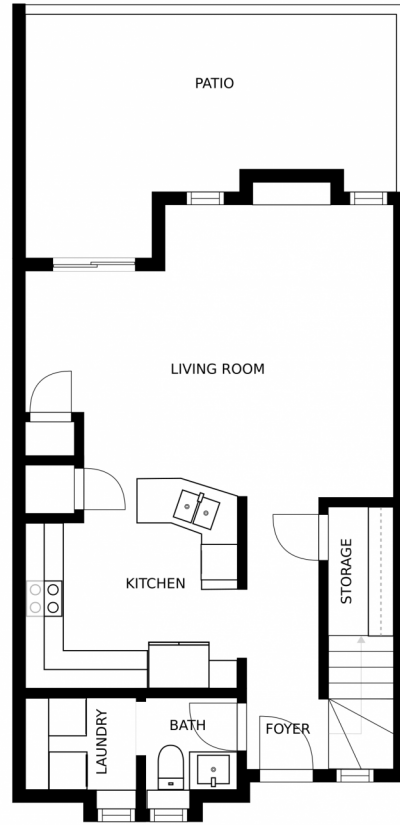
FLOOR 1
