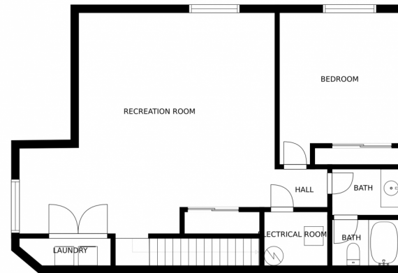
FLOOR 1
