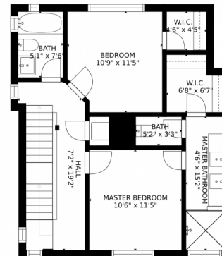
FLOOR 3
