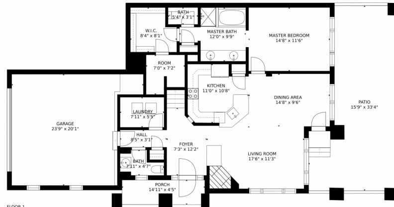
FLOOR 1
