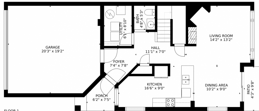
FLOOR 1
