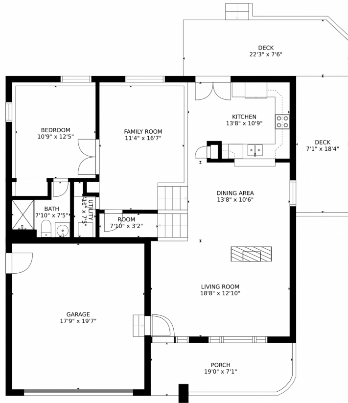
FLOOR 1
