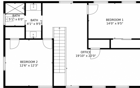
FLOOR 2
