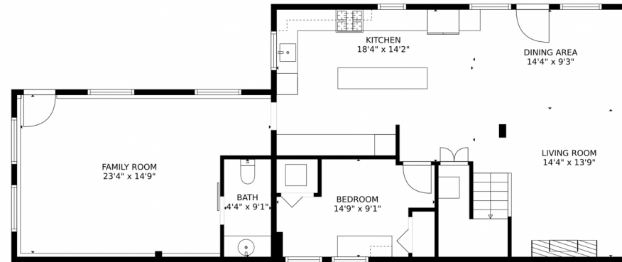
FLOOR 1
