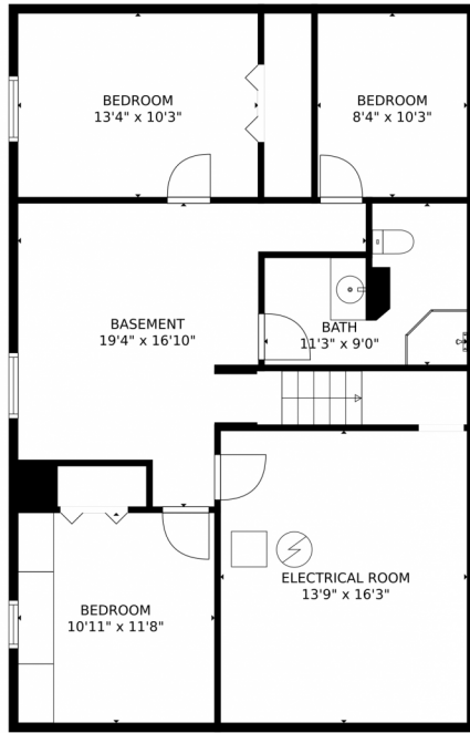
FLOOR 1
