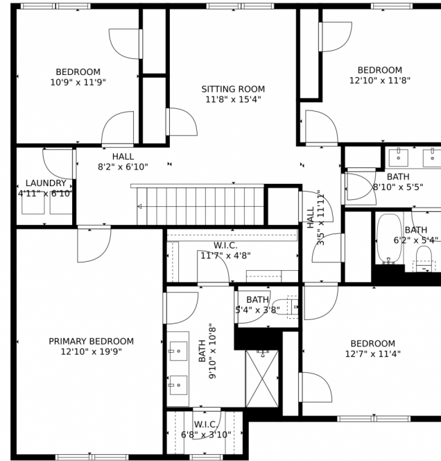
FLOOR 2
