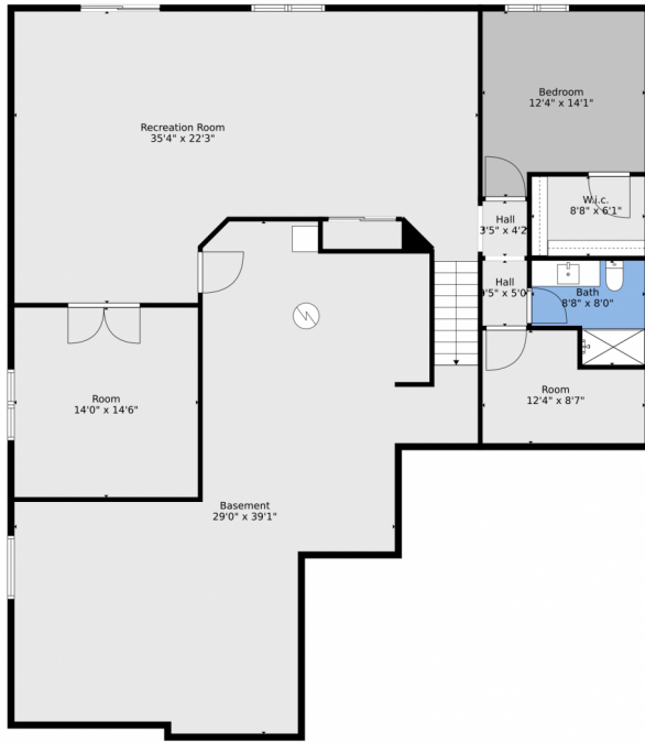
Floor 1
